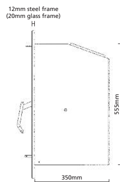
ARIEL 5 INSET STOVE DIMENSIONS Approx. weight 68kg
