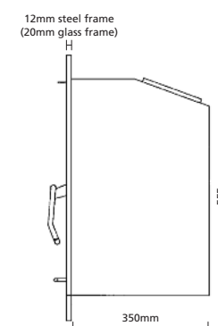
CALYPSO 5 INSET STOVE DIMENSIONS Approx. weight 85kg
