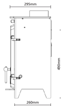
FDC 5 kW WIDE FREESTANDING STOVE DIMENSIONS Approx. weight 69kg
