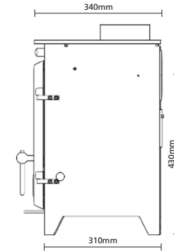
FDC 8 kW FREESTANDING STOVE DIMENSIONS Approx. weight 78kg
