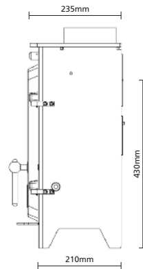
FDC 4 kW FREESTANDING STOVE DIMENSIONS Approx. weight 40kg
