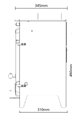
FDC 8 kW FREESTANDING STOVE DIMENSIONS Approx. weight 78kg
